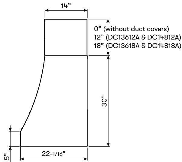
SIDE
